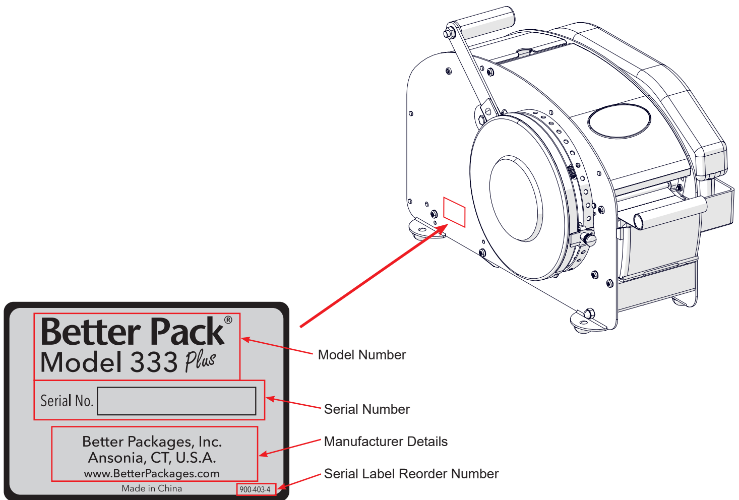
Figure 5: Machine Nameplate
